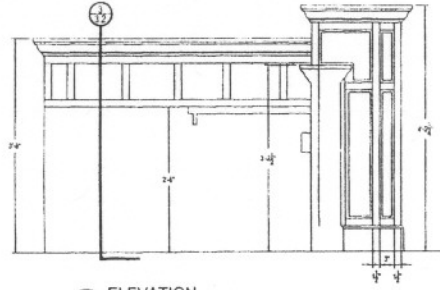
① ELEVATION COURTROOM 2 ROOM 107
