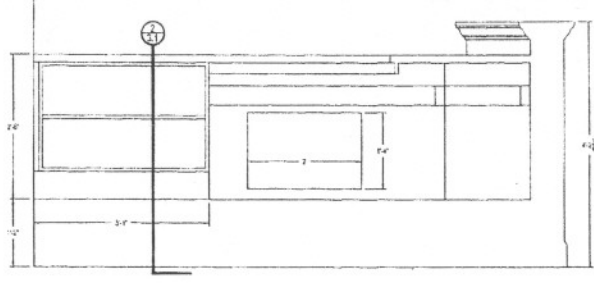
② ELEVATION COURTROOM 2 ROOM 107
