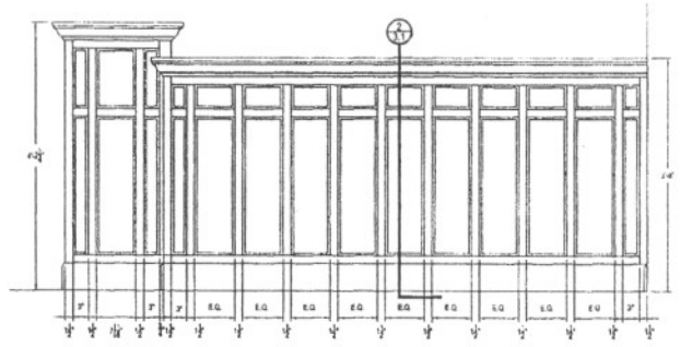
2 ELEVATION COURTROOM 2 ROOM 107
