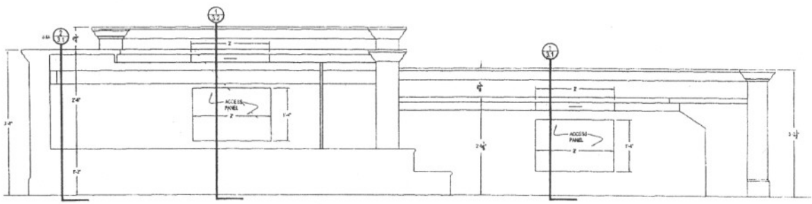
4 ELEVATION COURTROOM 2 ROOM 107
